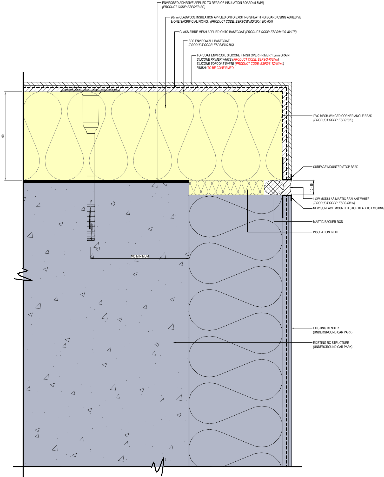
01 PLAN SECTION - RENDER - NEW TO EXISTING DETAIL Scale 1:1
